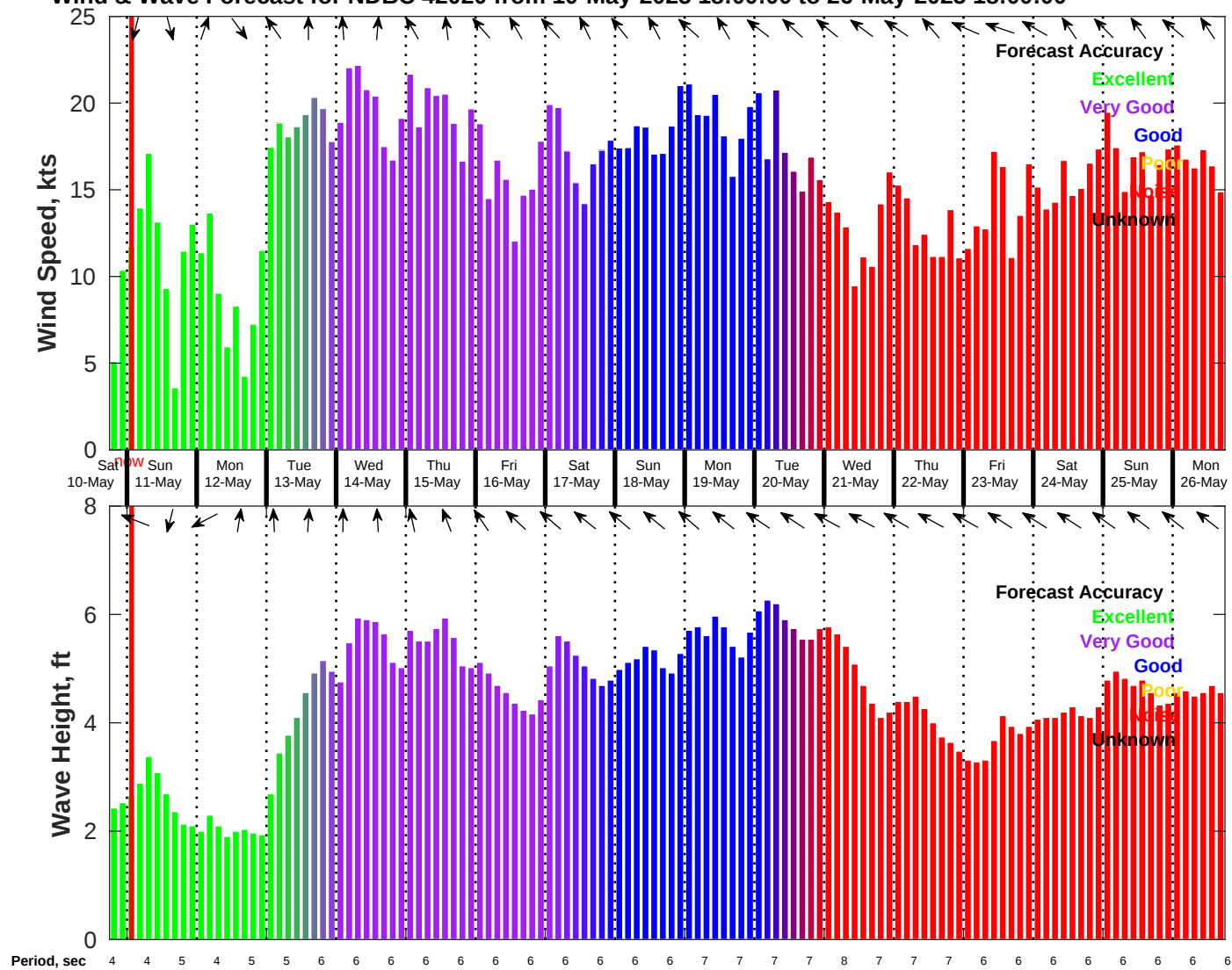
Wind & Wave Forecast for NDBC 42020 from 10-May-2025 18:00:00 to 26-May-2025 18:00:00
