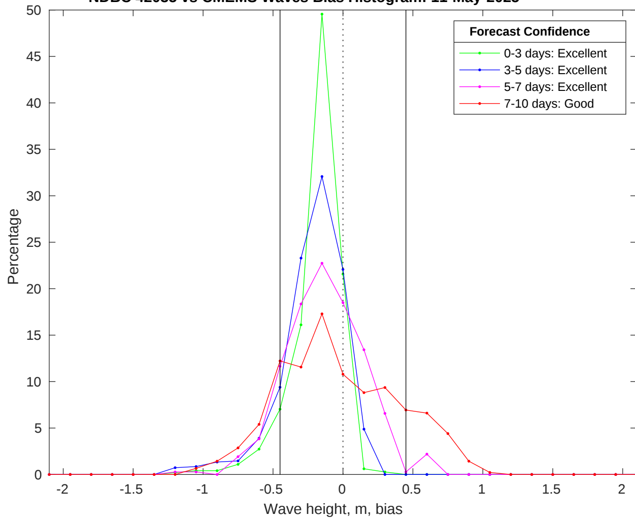
NDBC 42035 vs CMEMS Waves Bias Histogram: 11-May-2025
