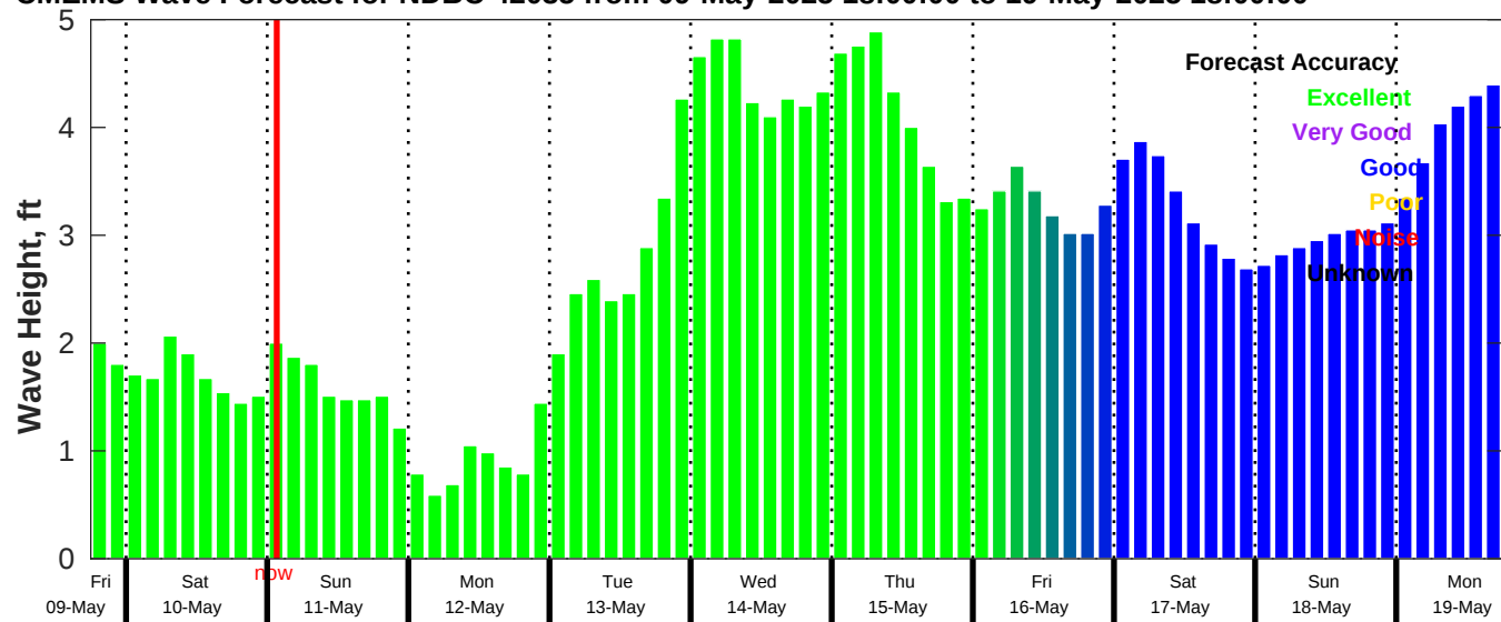
CMEMS Wave Forecast for NDBC 42035 from 09-May-2025 18:00:00 to 19-May-2025 18:00:00
