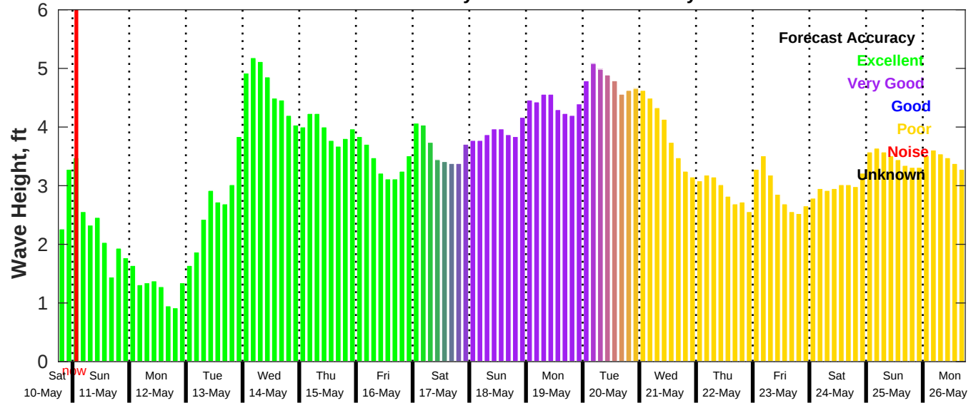
GFS Wave Forecast for NDBC 42035 from 10-May-2025 18:00:00 to 26-May-2025 18:00:00
