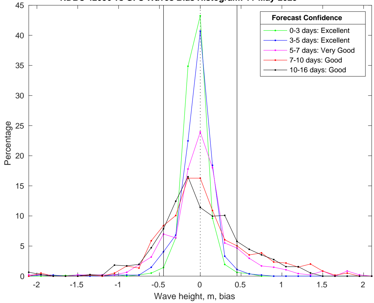
NDBC 42036 vs GFS Waves Bias Histogram: 11-May-2025
