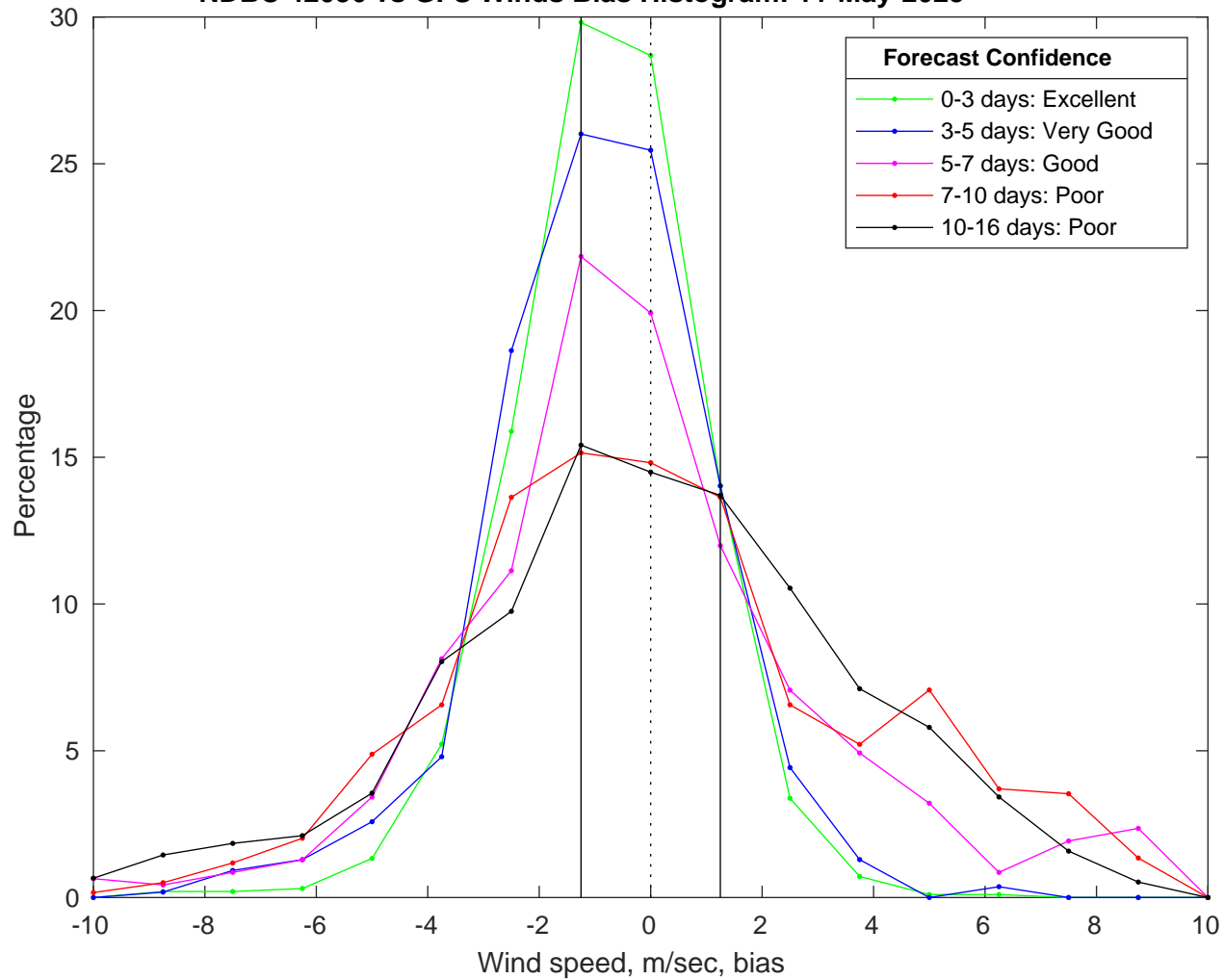
NDBC 42036 vs GFS Winds Bias Histogram: 11-May-2025
