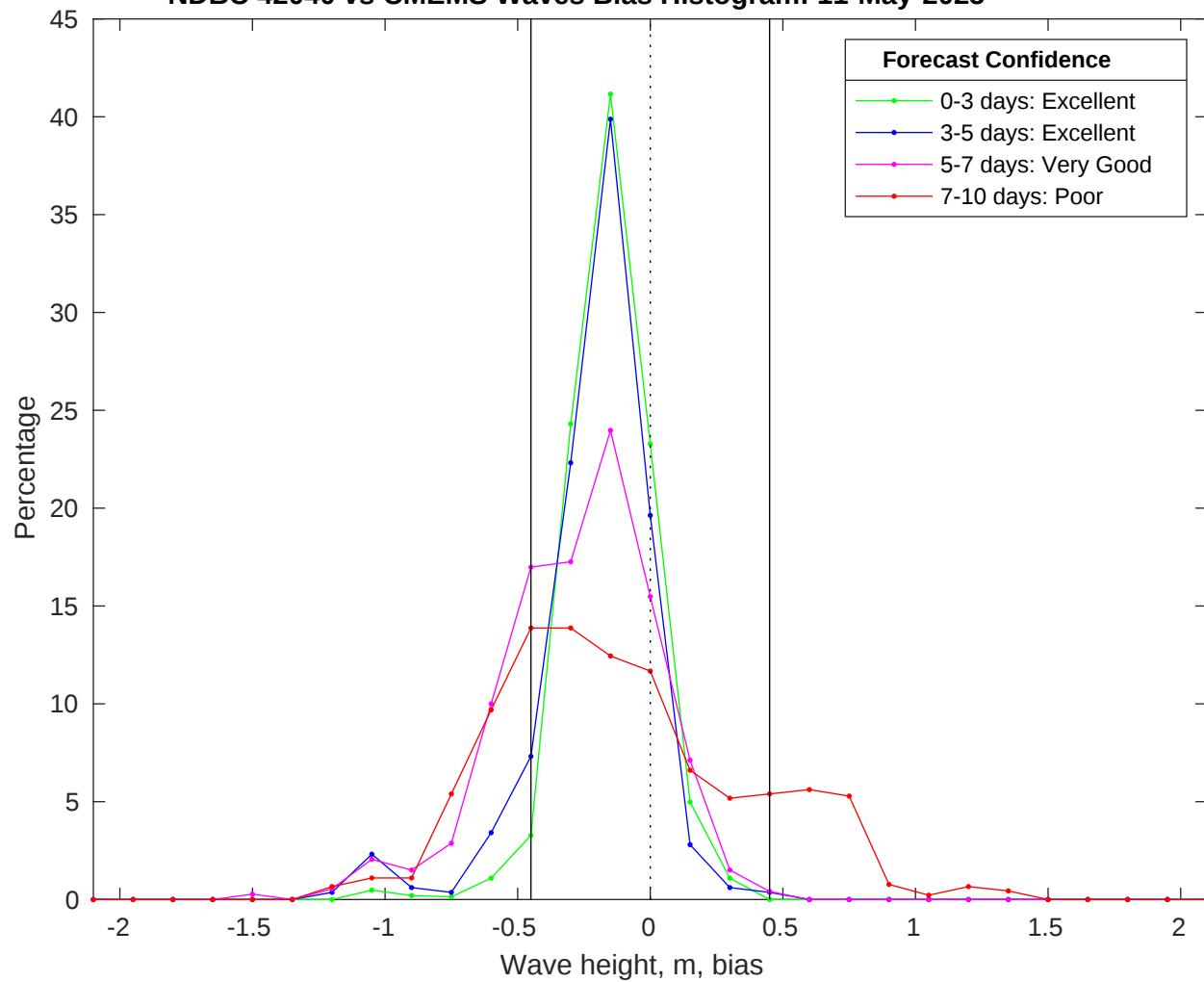
NDBC 42040 vs CMEMS Waves Bias Histogram: 11-May-2025
