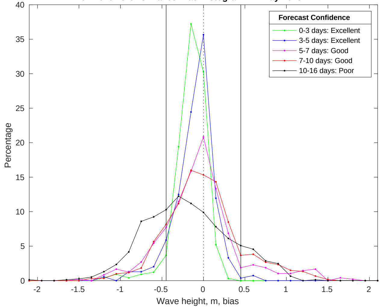
NDBC 42040 vs GFS Waves Bias Histogram: 11-May-2025
