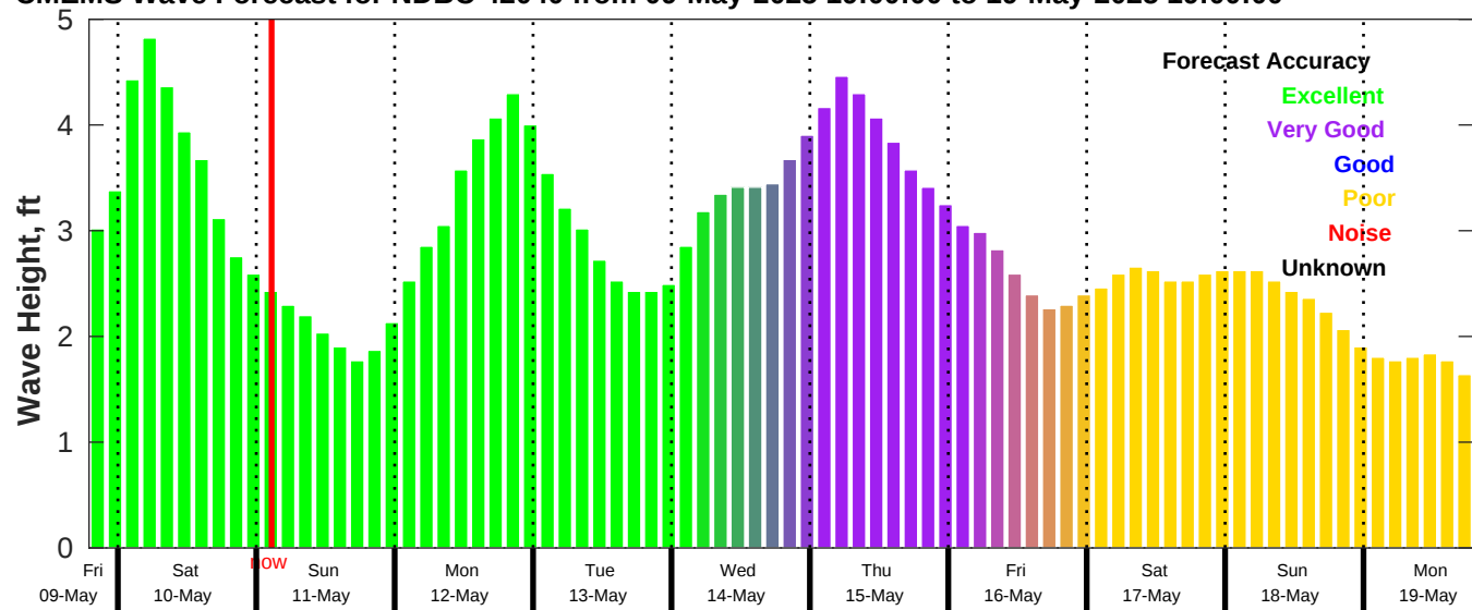
CMEMS Wave Forecast for NDBC 42040 from 09-May-2025 19:00:00 to 19-May-2025 19:00:00
