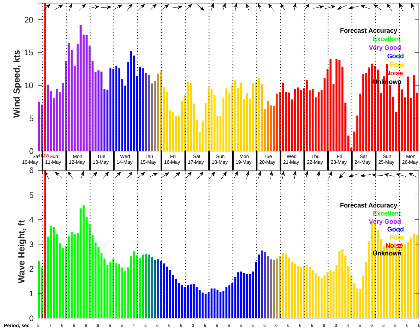
Wind & Wave Forecast for NDBC 42040 from 10-May-2025 19:00:00 to 26-May-2025 19:00:00
