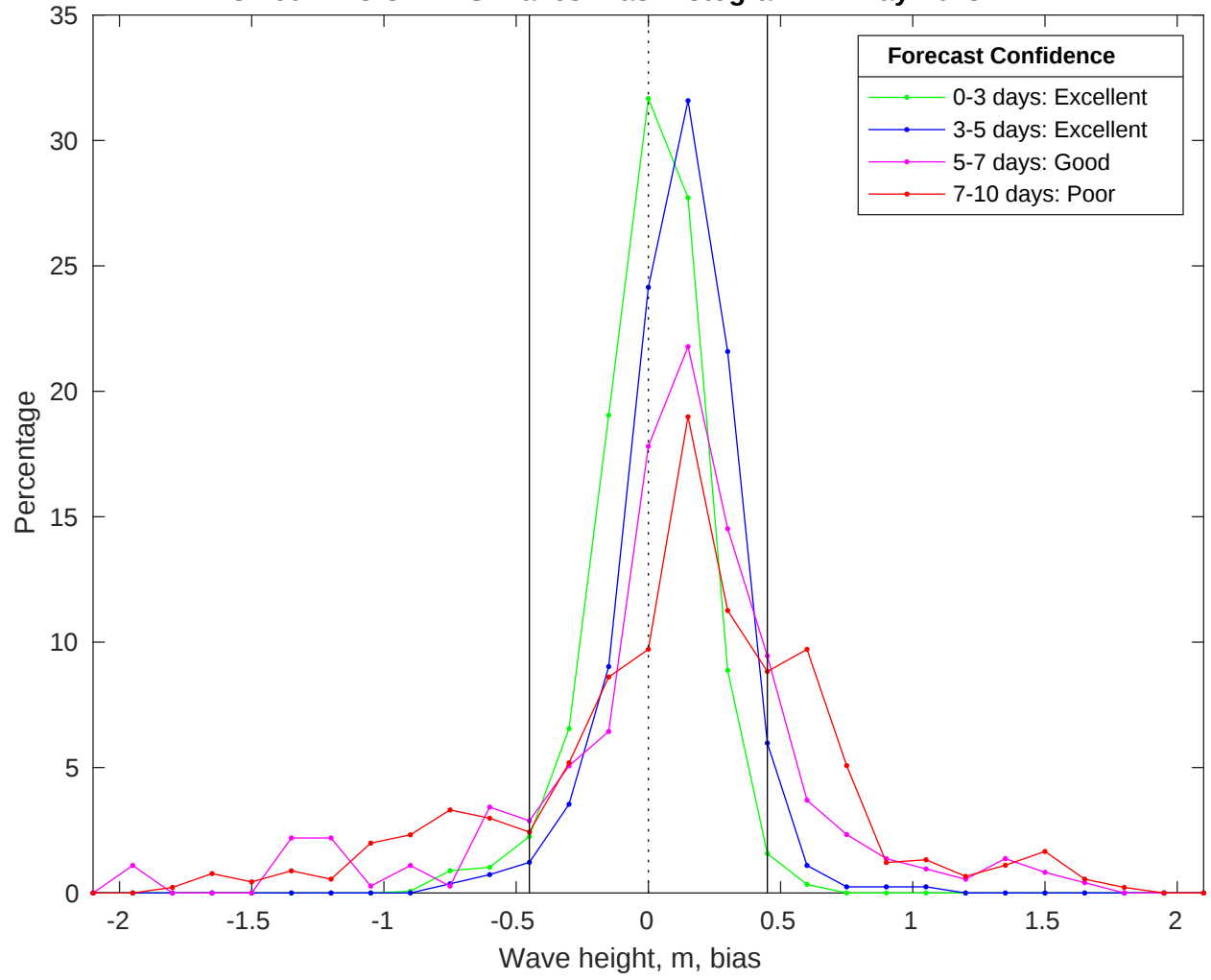
NDBC 46011 vs CMEMS Waves Bias Histogram: 11-May-2025
