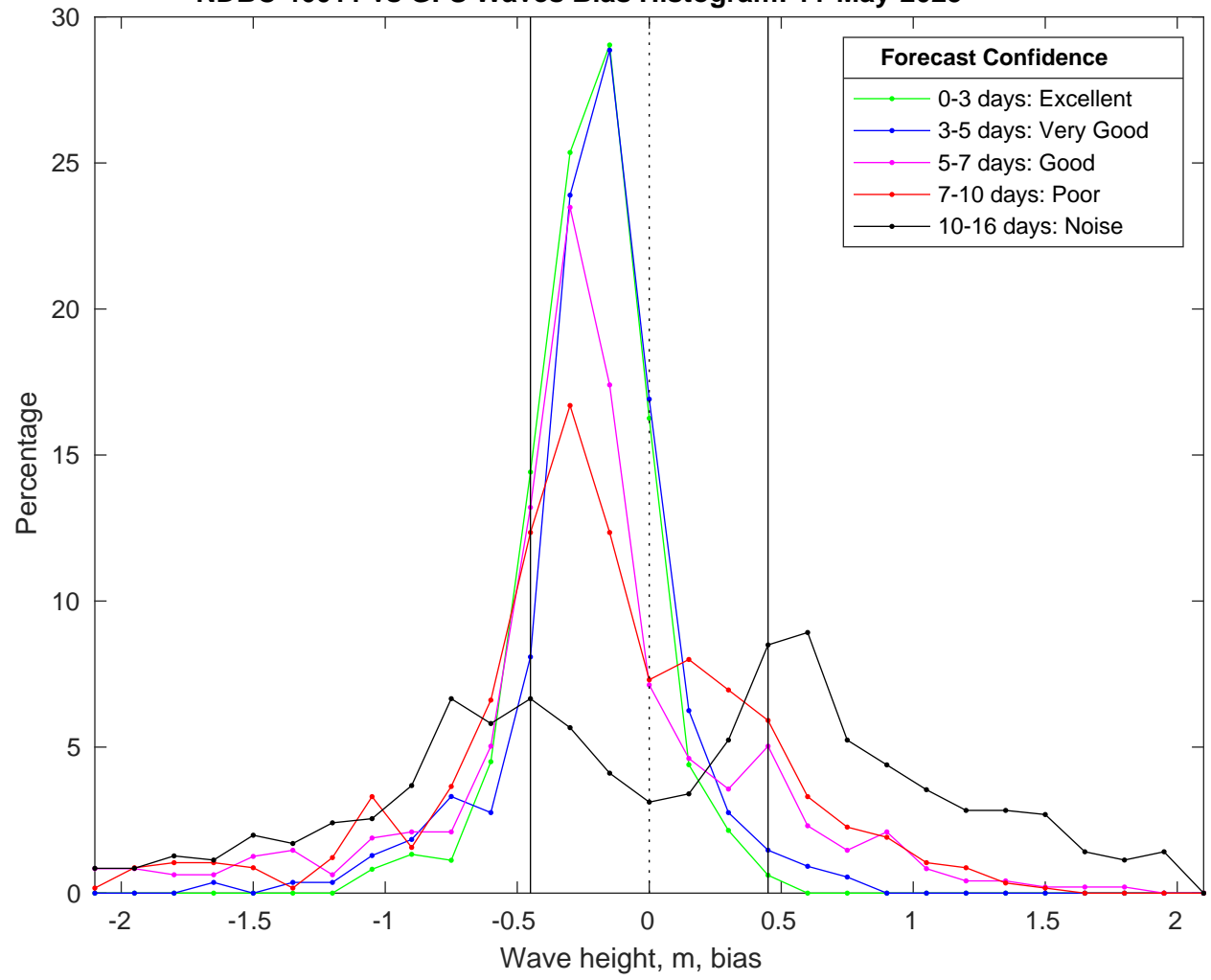
NDBC 46011 vs GFS Waves Bias Histogram: 11-May-2025
