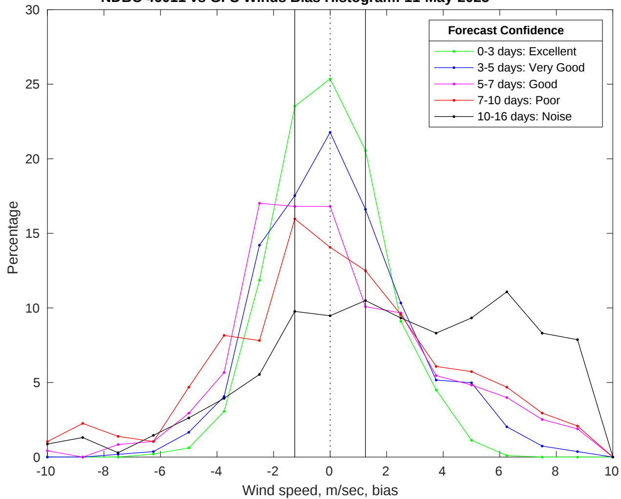
NDBC 46011 vs GFS Winds Bias Histogram: 11-May-2025
