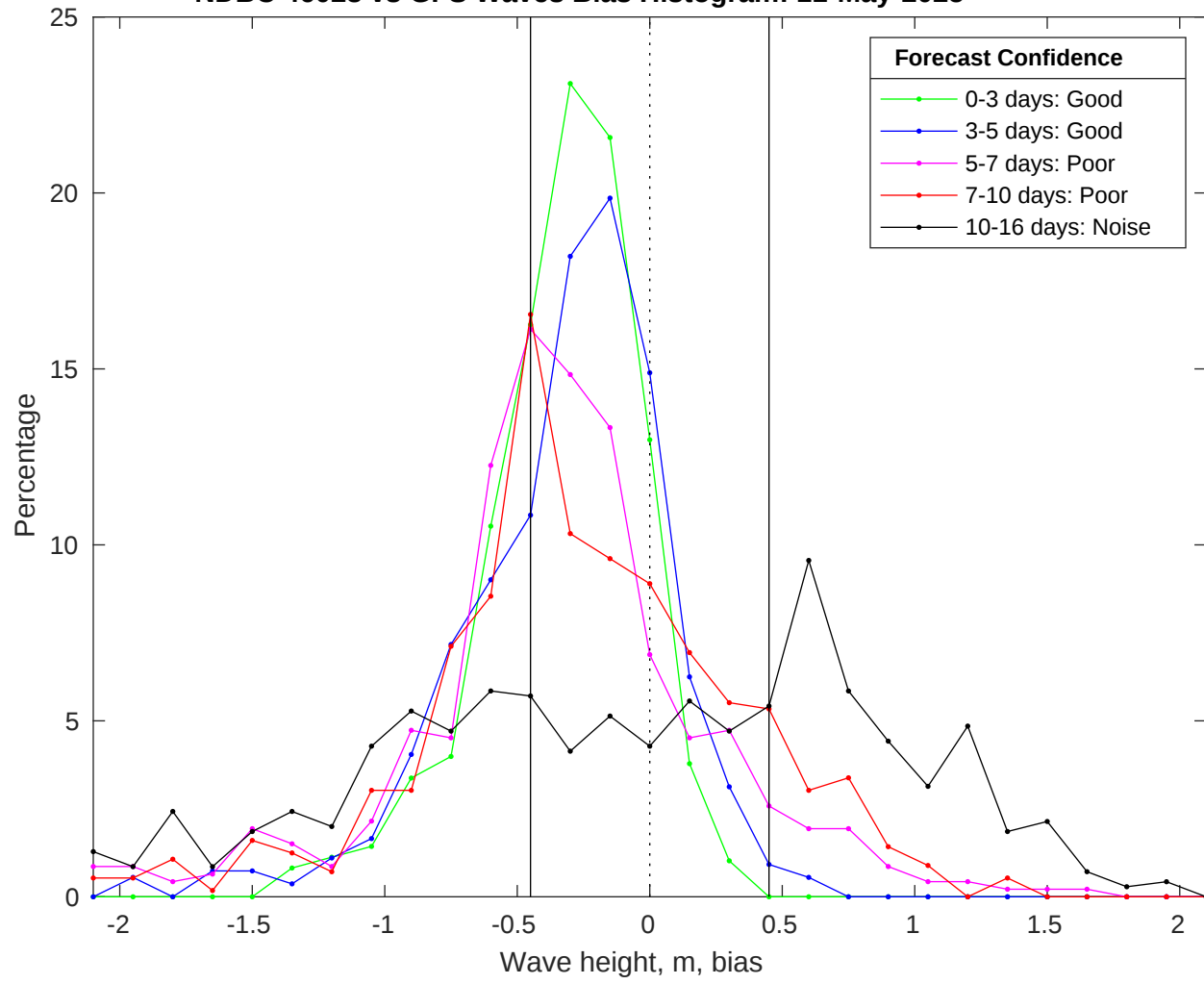
NDBC 46028 vs GFS Waves Bias Histogram: 11-May-2025
