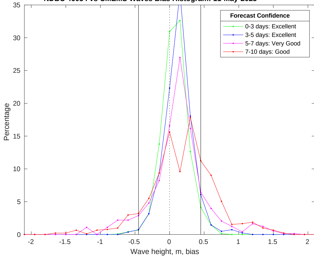
NDBC 46054 vs CMEMS Waves Bias Histogram: 11-May-2025
