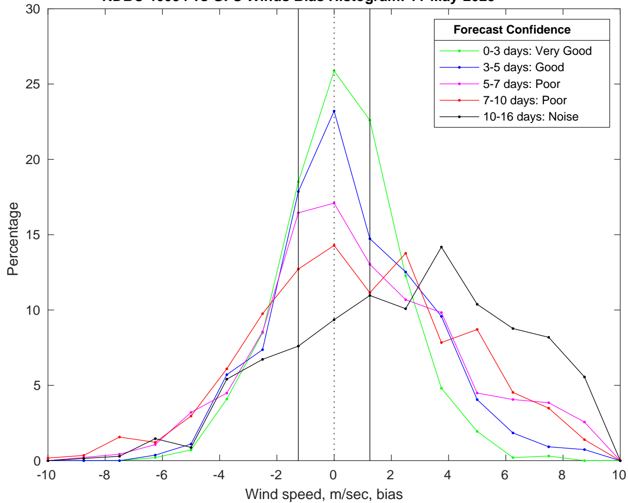
NDBC 46054 vs GFS Winds Bias Histogram: 11-May-2025
