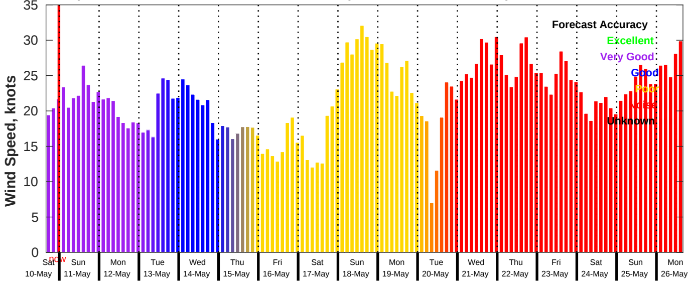
GFS Wind Speed Forecast for NDBC 46054 from 10-May-2025 16:00:00 to 26-May-2025 16:00:00
