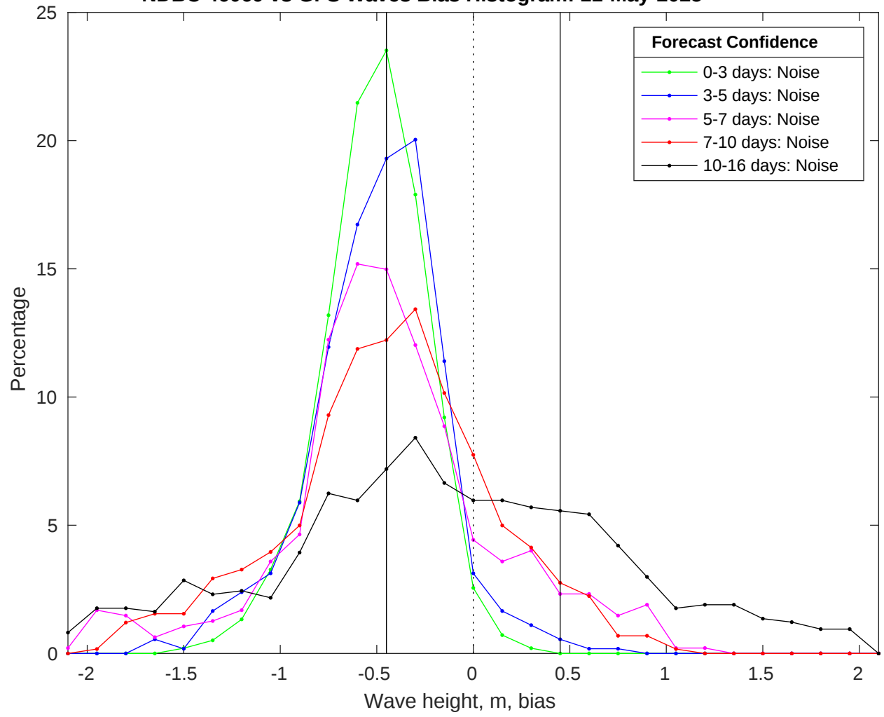
NDBC 46069 vs GFS Waves Bias Histogram: 11-May-2025
