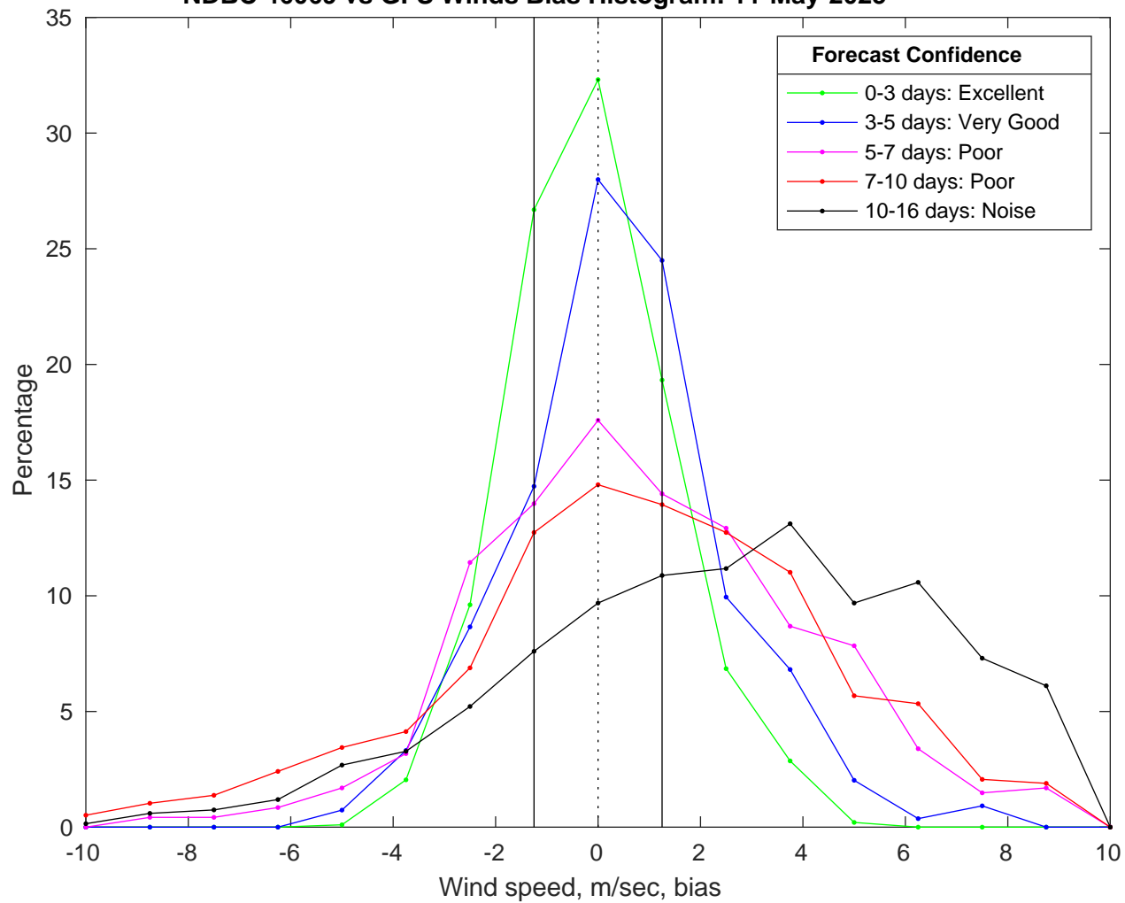
NDBC 46069 vs GFS Winds Bias Histogram: 11-May-2025
