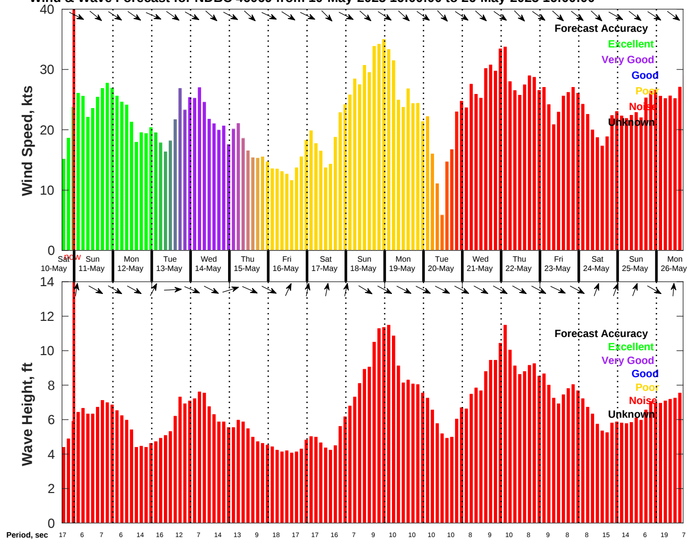
Wind & Wave Forecast for NDBC 46069 from 10-May-2025 16:00:00 to 26-May-2025 16:00:00
