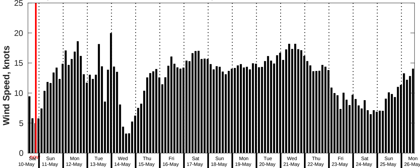
GFS Wind Speed Forecast for NDBC 51209 from 10-May-2025 13:00:00 to 26-May-2025 13:00:00
