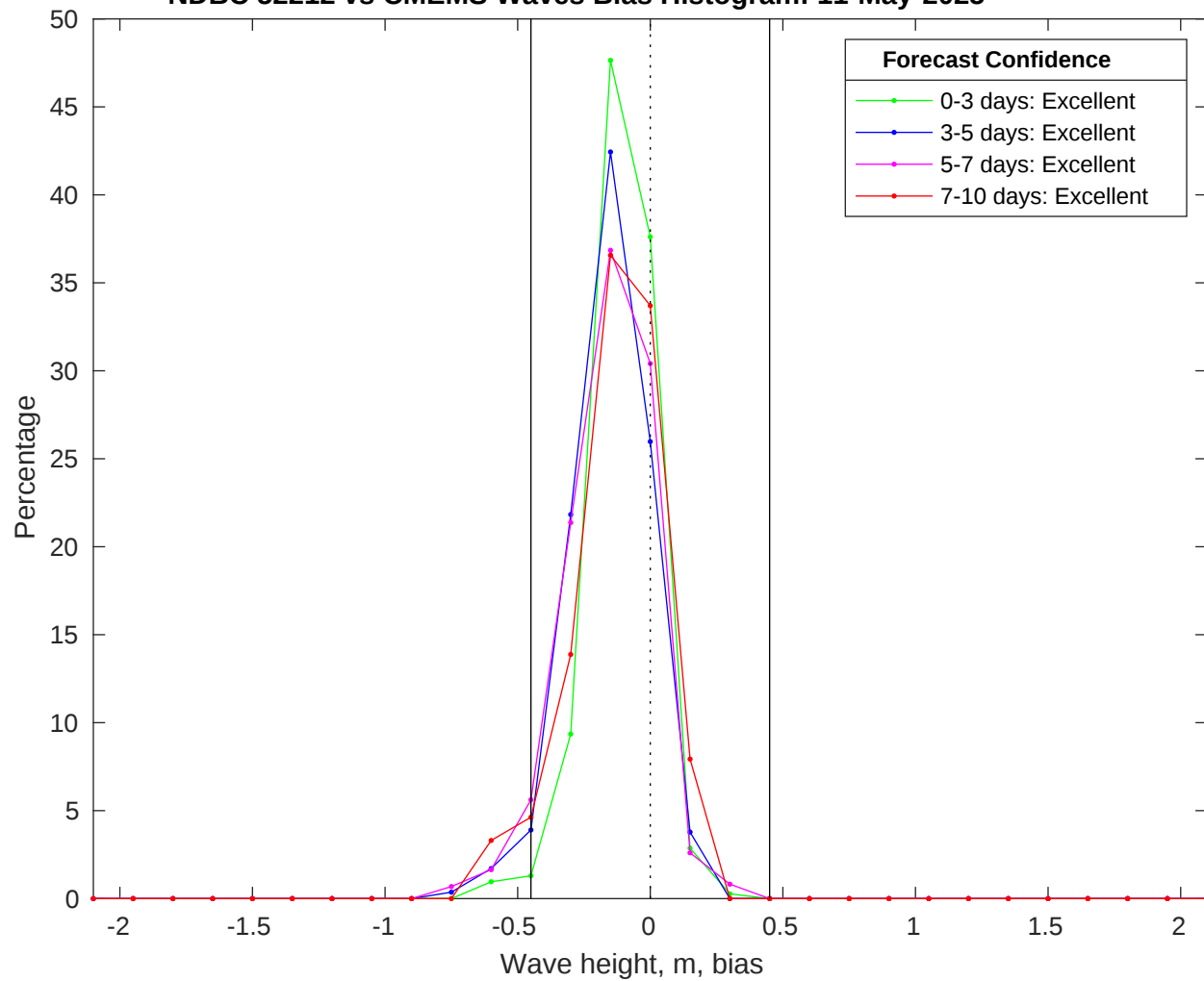
NDBC 52212 vs CMEMS Waves Bias Histogram: 11-May-2025
