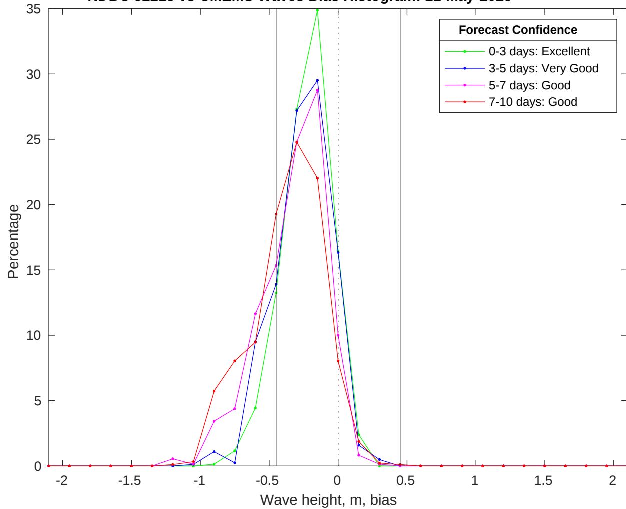
NDBC 52213 vs CMEMS Waves Bias Histogram: 11-May-2025
