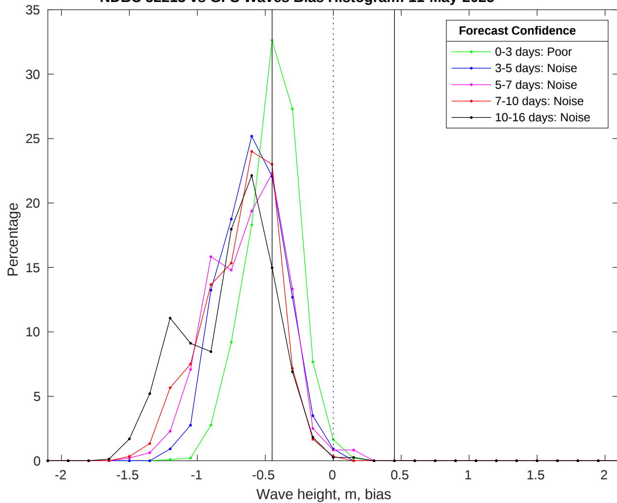
NDBC 52213 vs GFS Waves Bias Histogram: 11-May-2025
