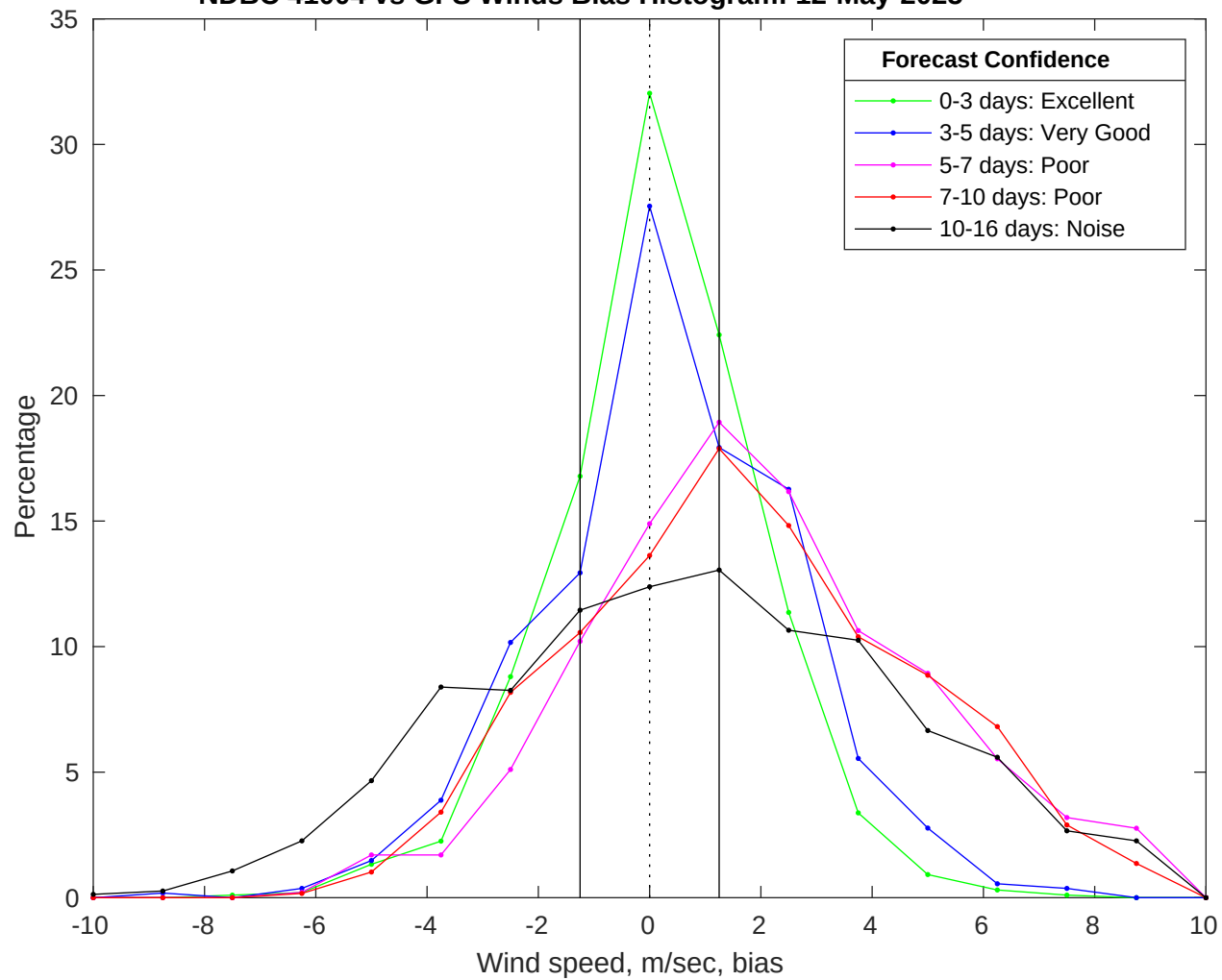
NDBC 41004 vs GFS Winds Bias Histogram: 12-May-2025
