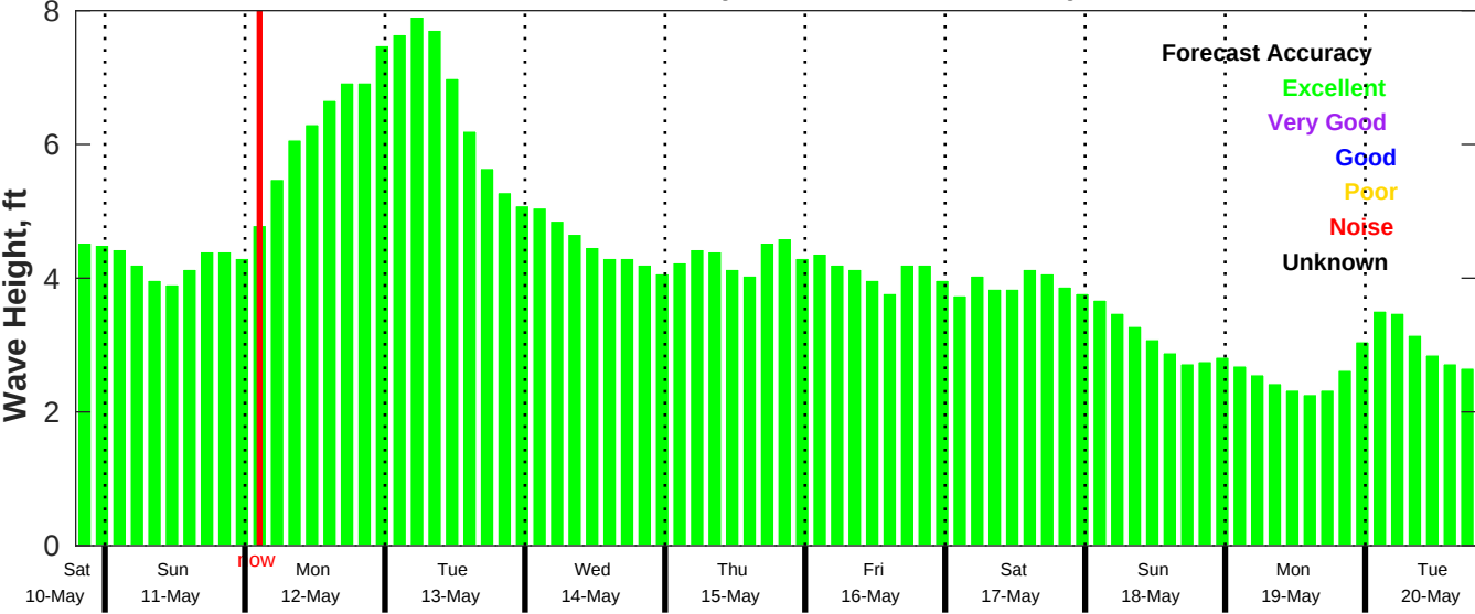
CMEMS Wave Forecast for NDBC 41004 from 10-May-2025 19:00:00 to 20-May-2025 19:00:00
