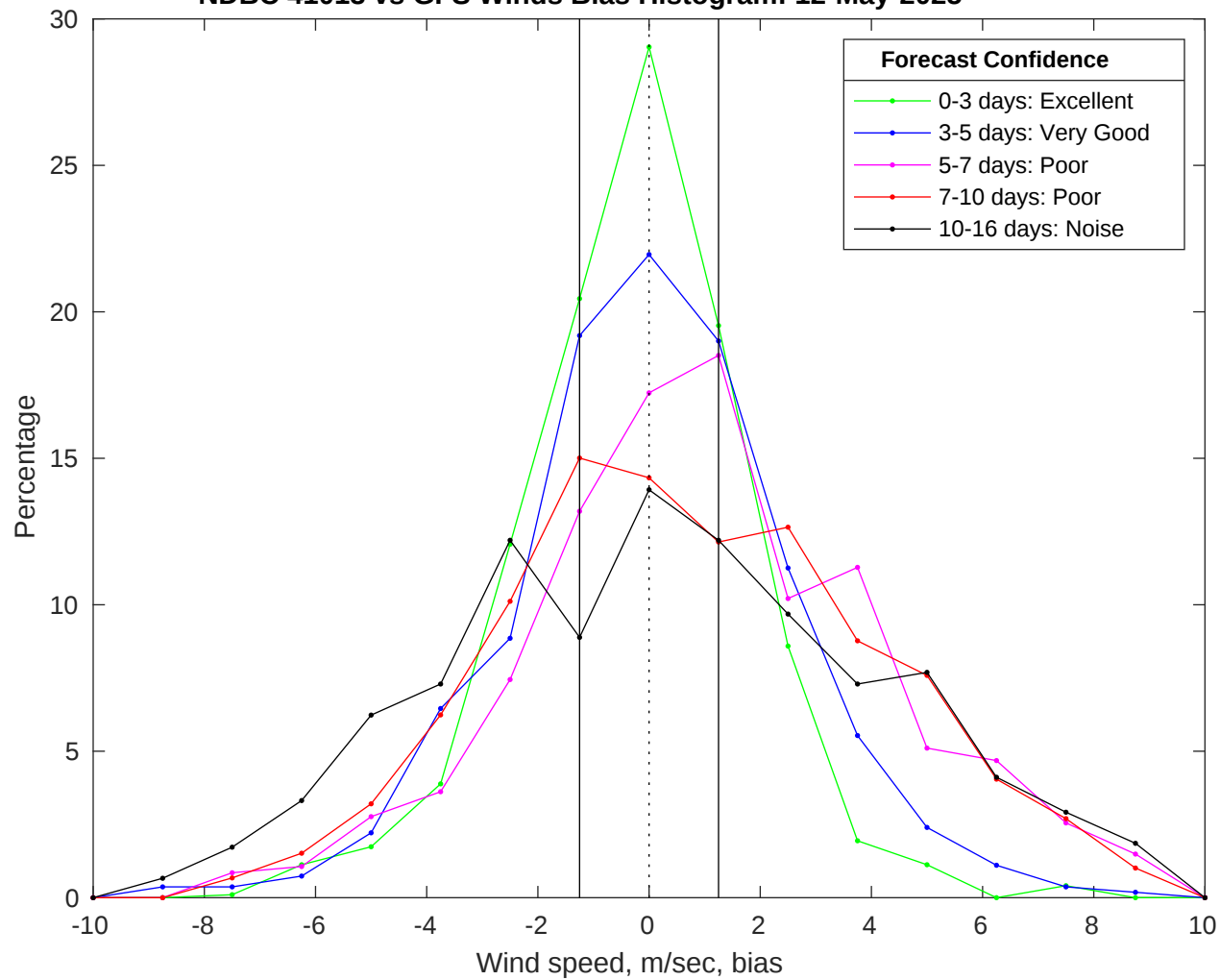
NDBC 41013 vs GFS Winds Bias Histogram: 12-May-2025
