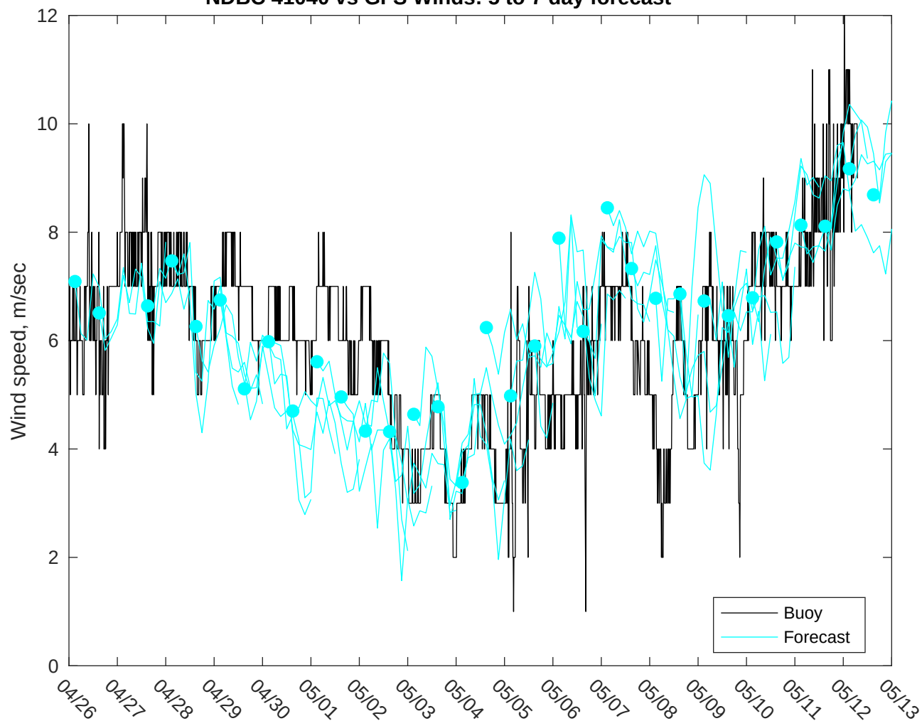
NDBC 41040 vs GFS Winds: 5 to 7 day forecast
