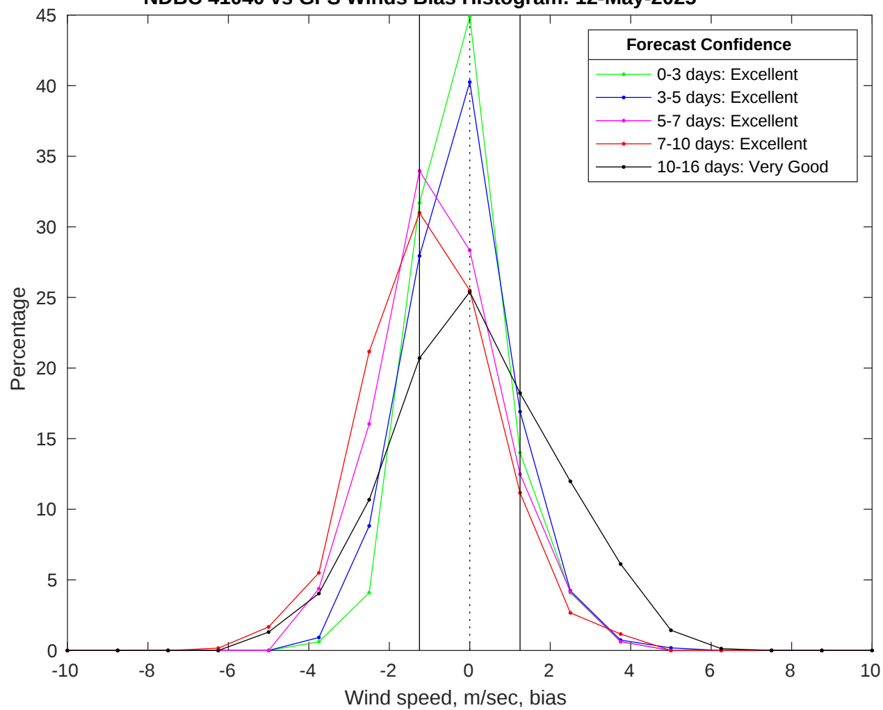
NDBC 41040 vs GFS Winds Bias Histogram: 12-May-2025
