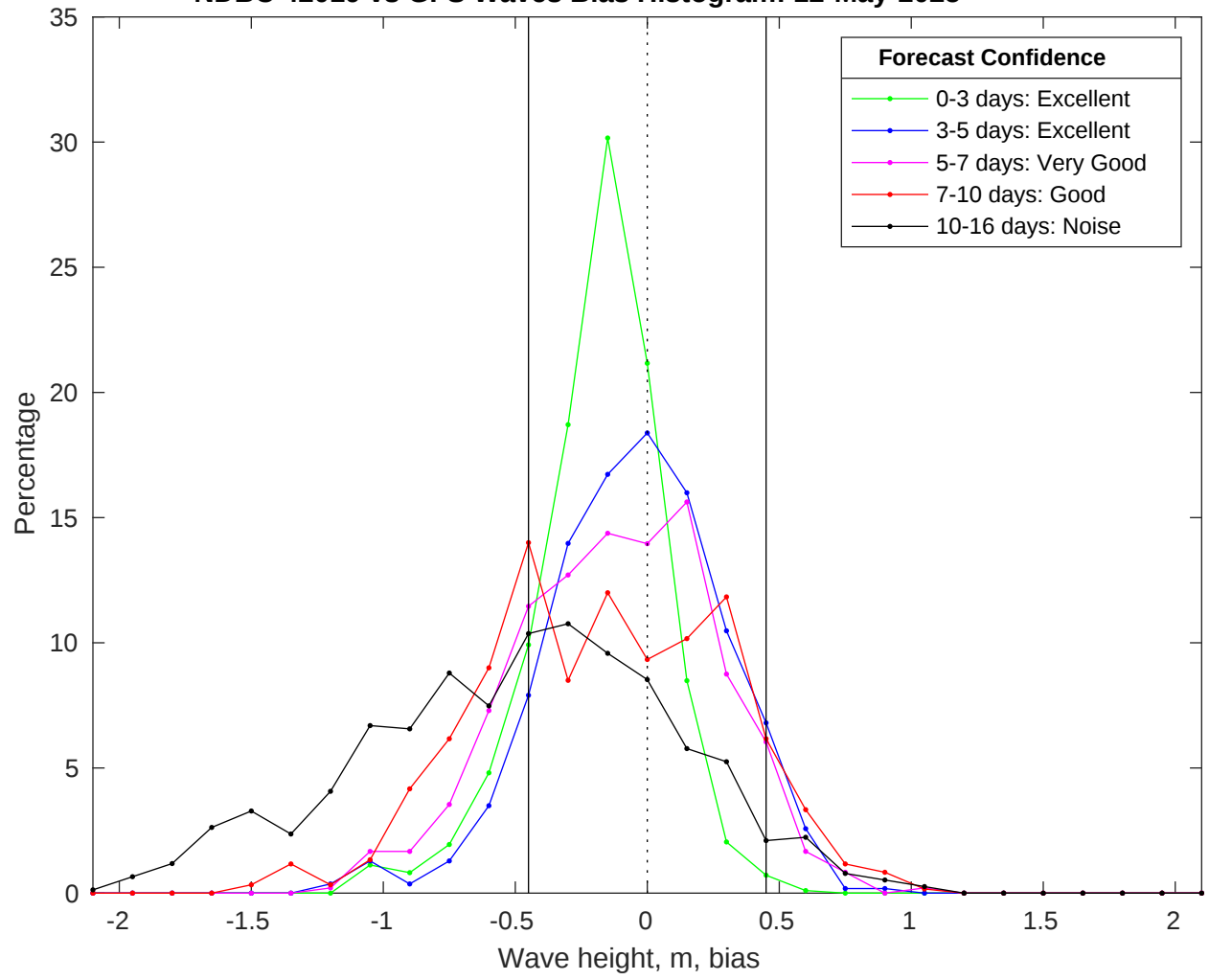
NDBC 42019 vs GFS Waves Bias Histogram: 12-May-2025
