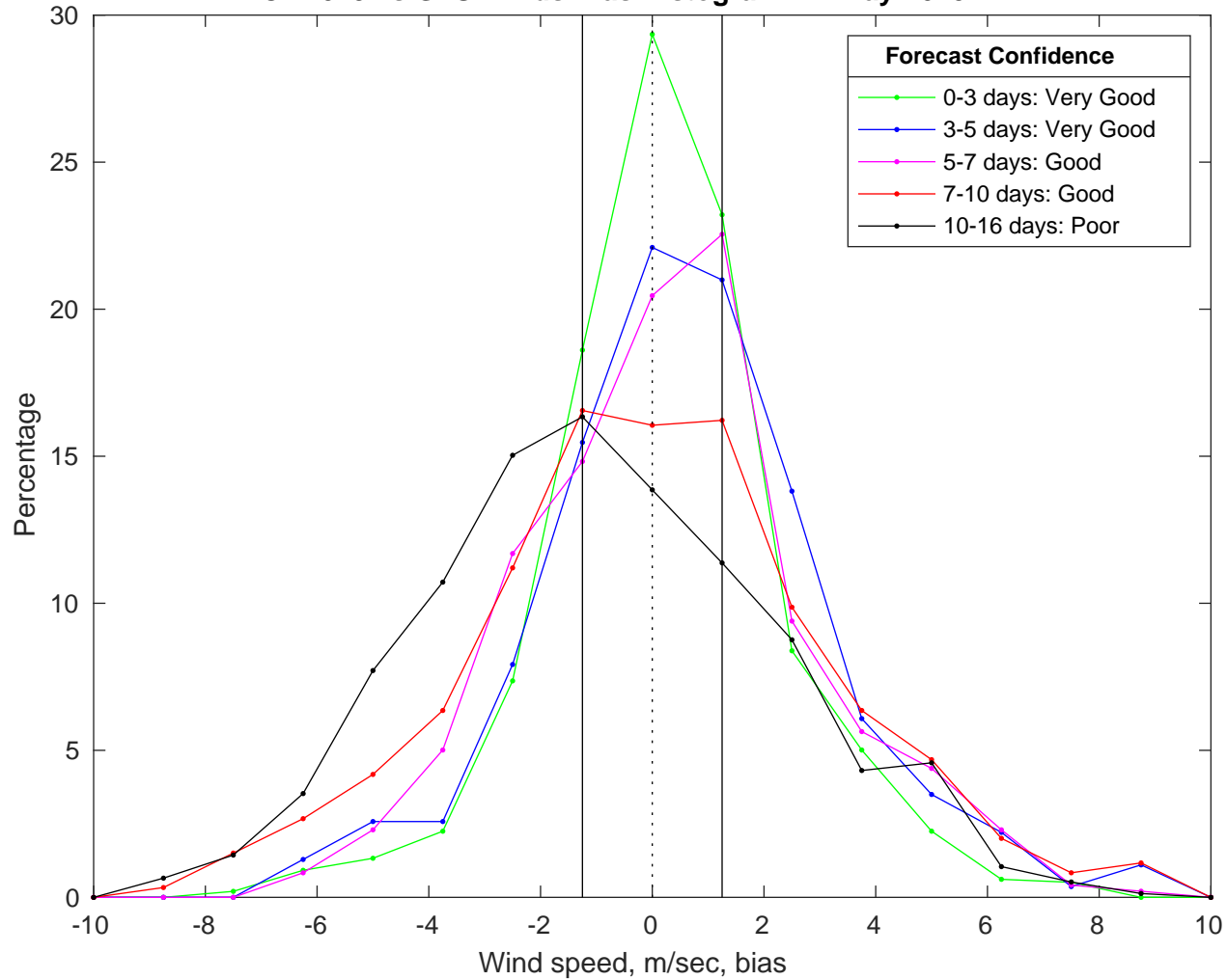
NDBC 42019 vs GFS Winds Bias Histogram: 12-May-2025
