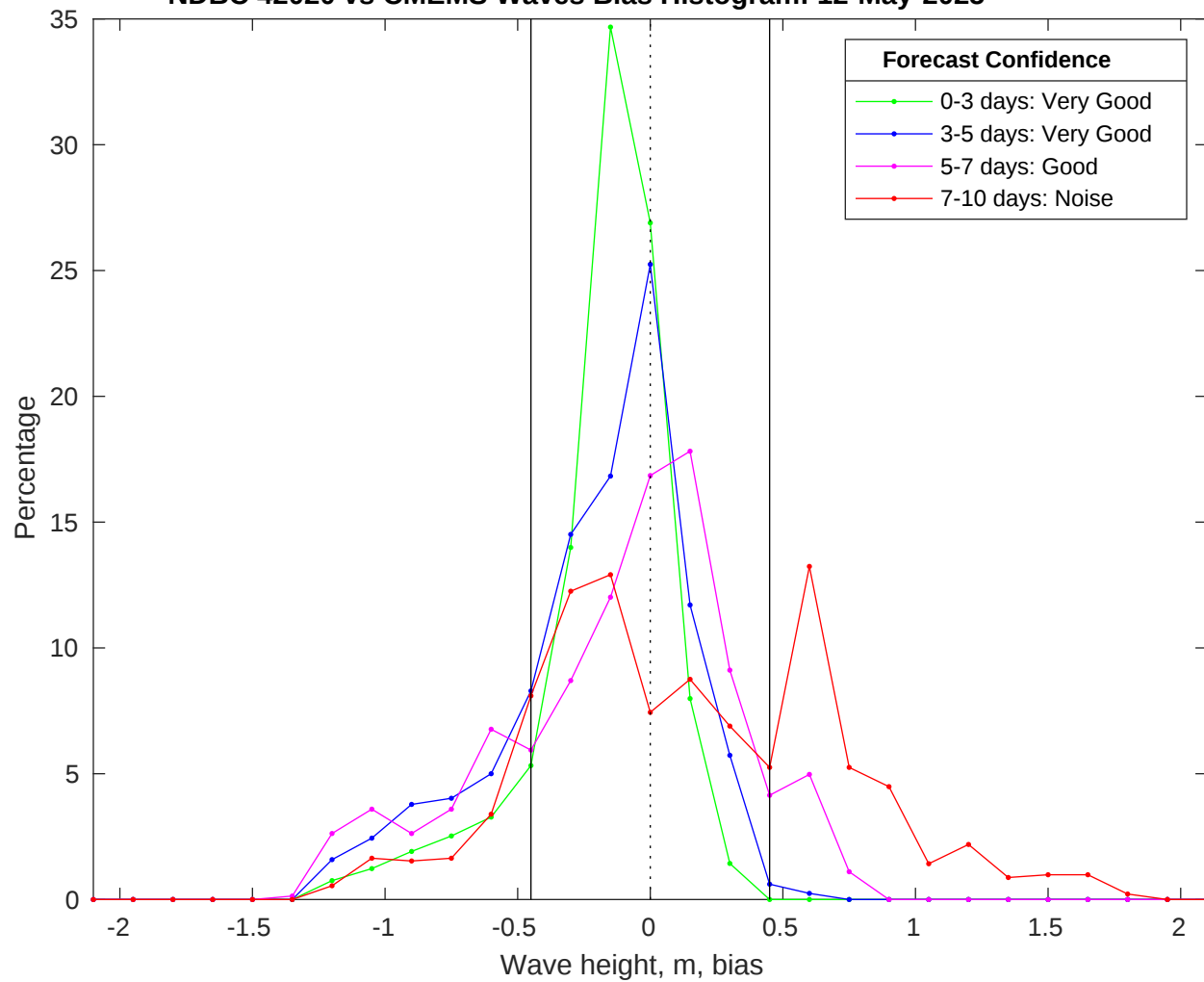
NDBC 42020 vs CMEMS Waves Bias Histogram: 12-May-2025
