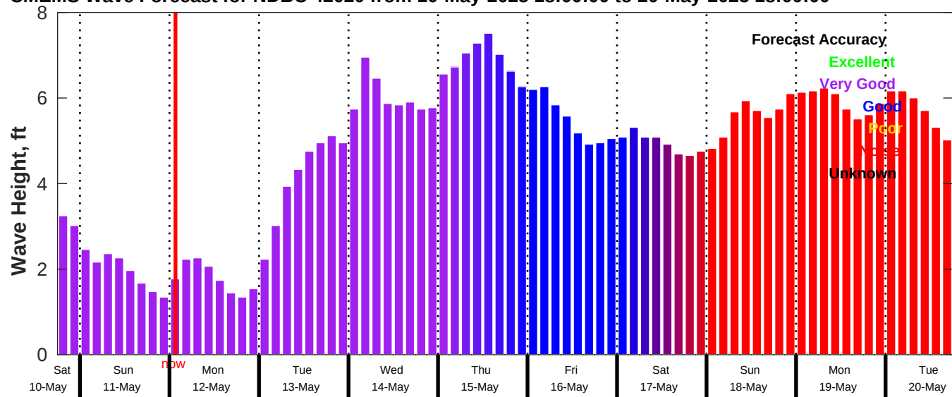
CMEMS Wave Forecast for NDBC 42020 from 10-May-2025 18:00:00 to 20-May-2025 18:00:00
