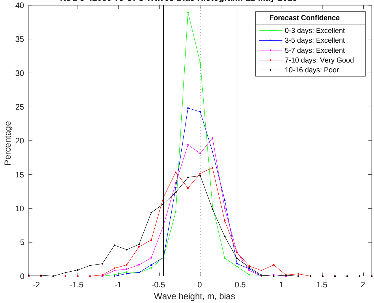
NDBC 42035 vs GFS Waves Bias Histogram: 12-May-2025
