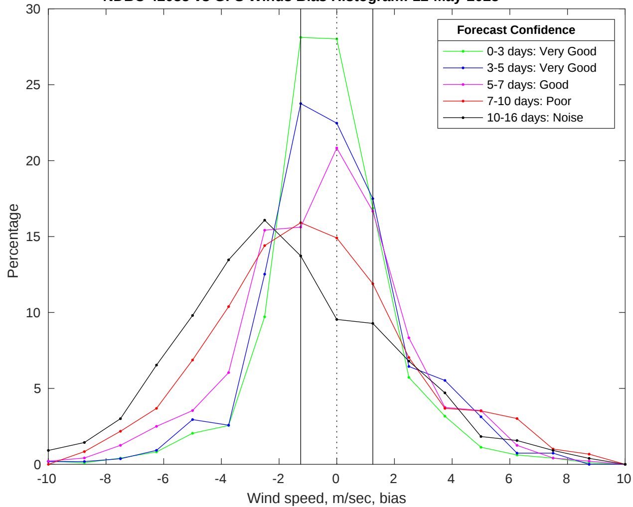
NDBC 42035 vs GFS Winds Bias Histogram: 12-May-2025
