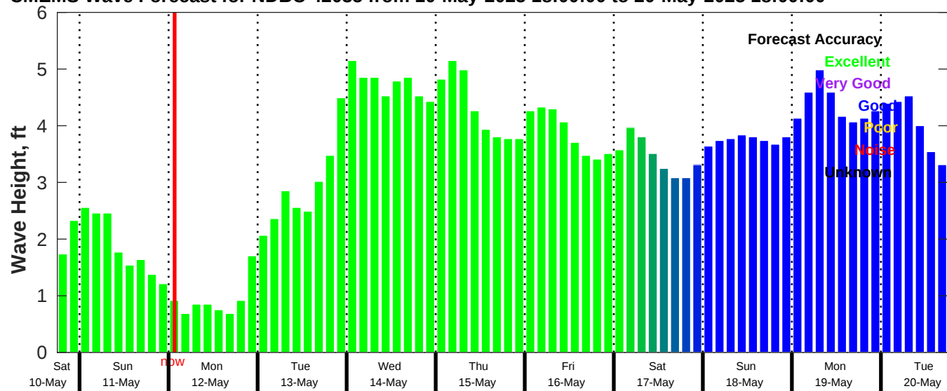
CMEMS Wave Forecast for NDBC 42035 from 10-May-2025 18:00:00 to 20-May-2025 18:00:00
