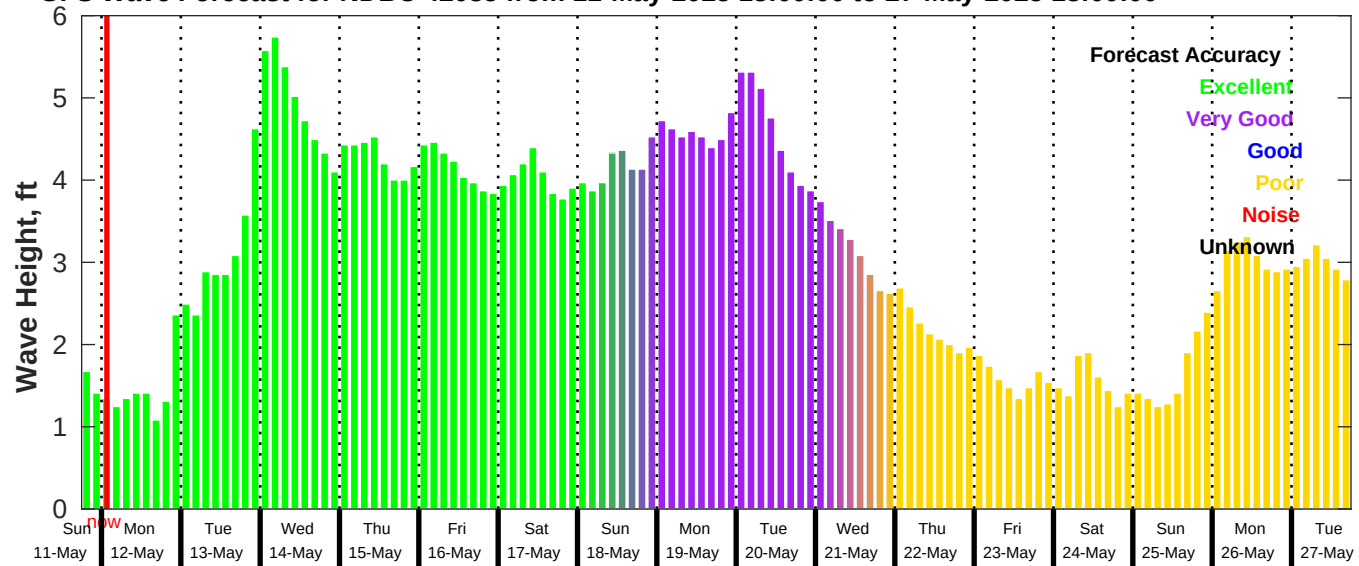
GFS Wave Forecast for NDBC 42035 from 11-May-2025 18:00:00 to 27-May-2025 18:00:00
