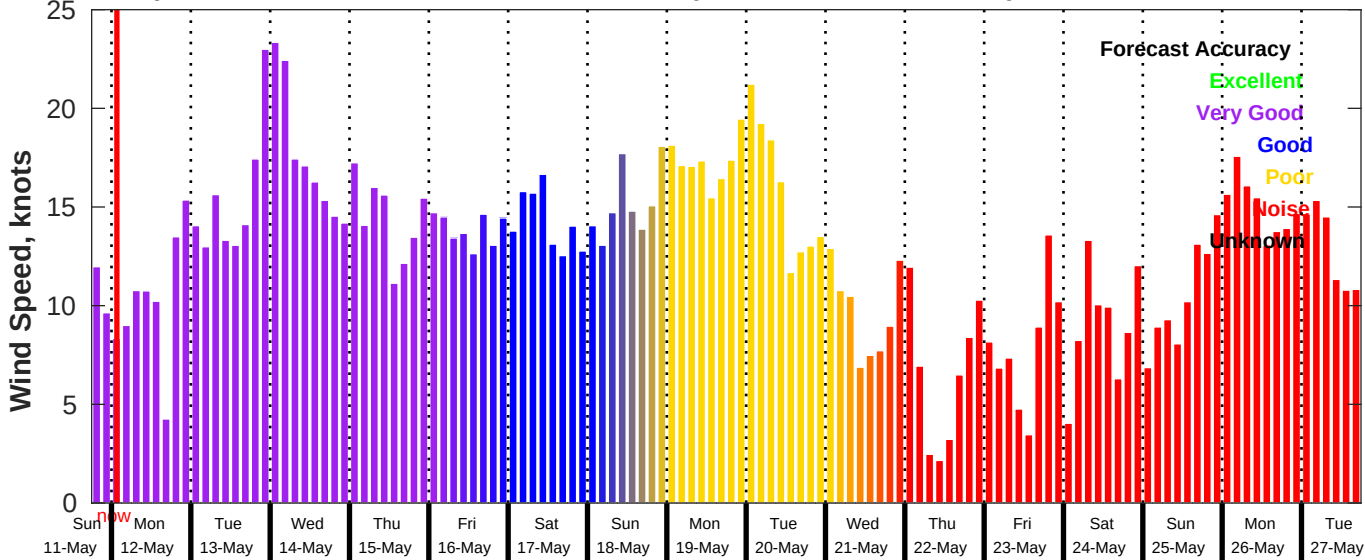
GFS Wind Speed Forecast for NDBC 42035 from 11-May-2025 18:00:00 to 27-May-2025 18:00:00
