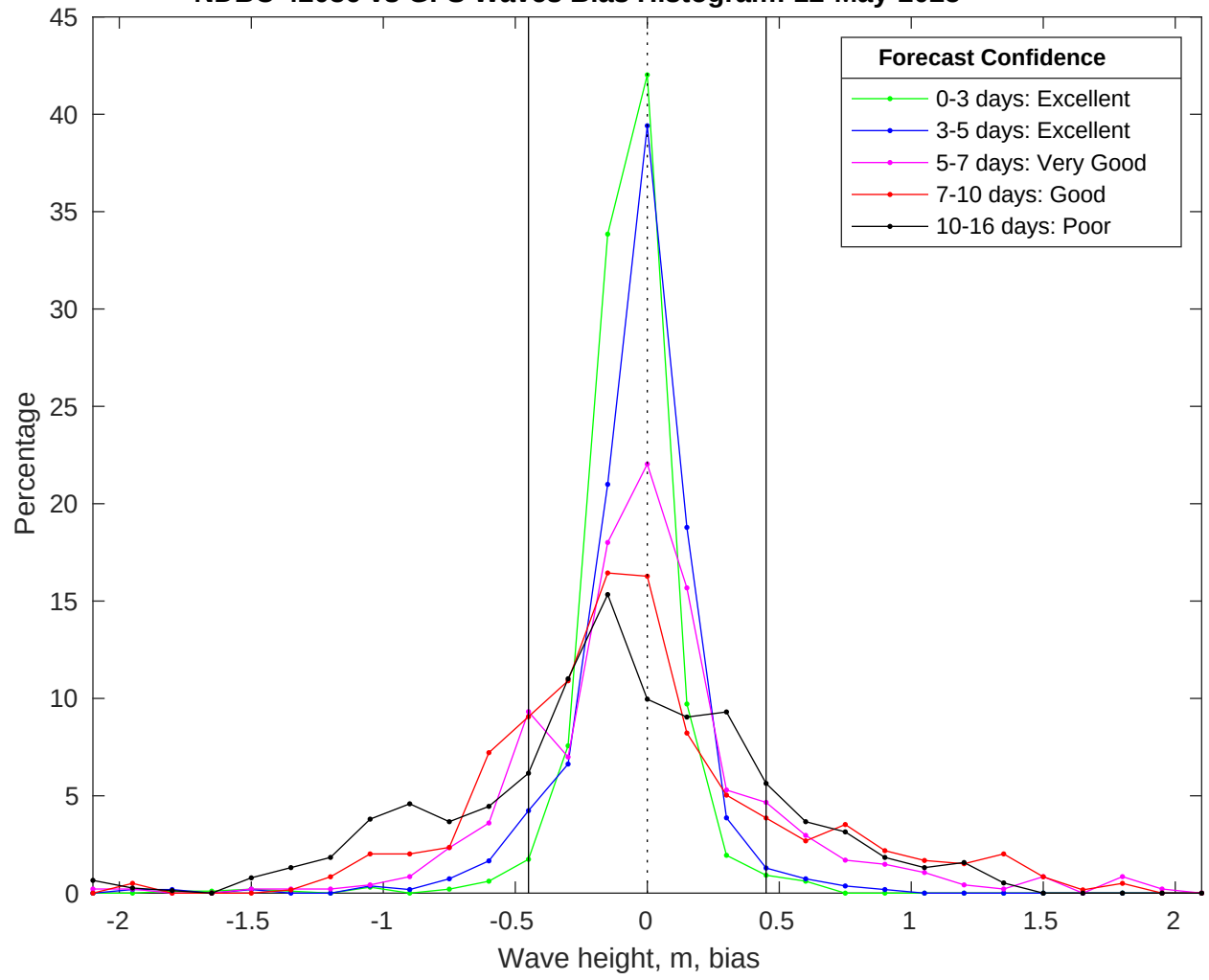
NDBC 42036 vs GFS Waves Bias Histogram: 12-May-2025
