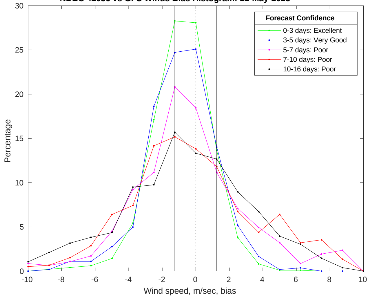
NDBC 42036 vs GFS Winds Bias Histogram: 12-May-2025
