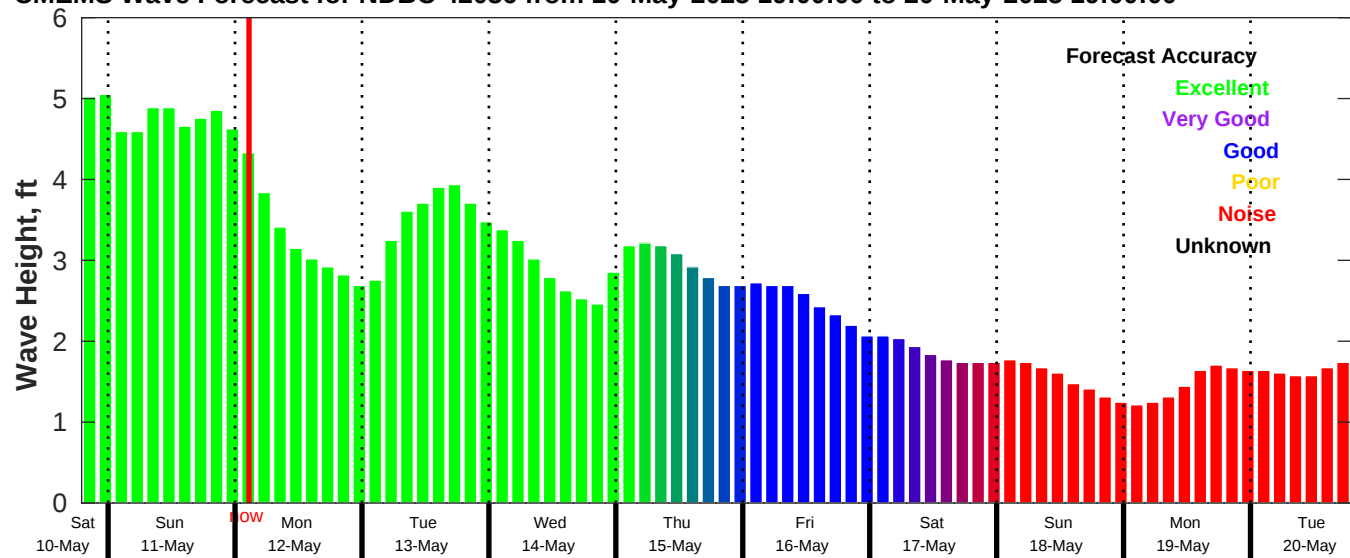
CMEMS Wave Forecast for NDBC 42036 from 10-May-2025 19:00:00 to 20-May-2025 19:00:00
