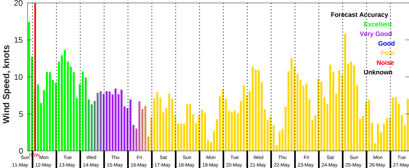
GFS Wind Speed Forecast for NDBC 42036 from 11-May-2025 19:00:00 to 27-May-2025 19:00:00
