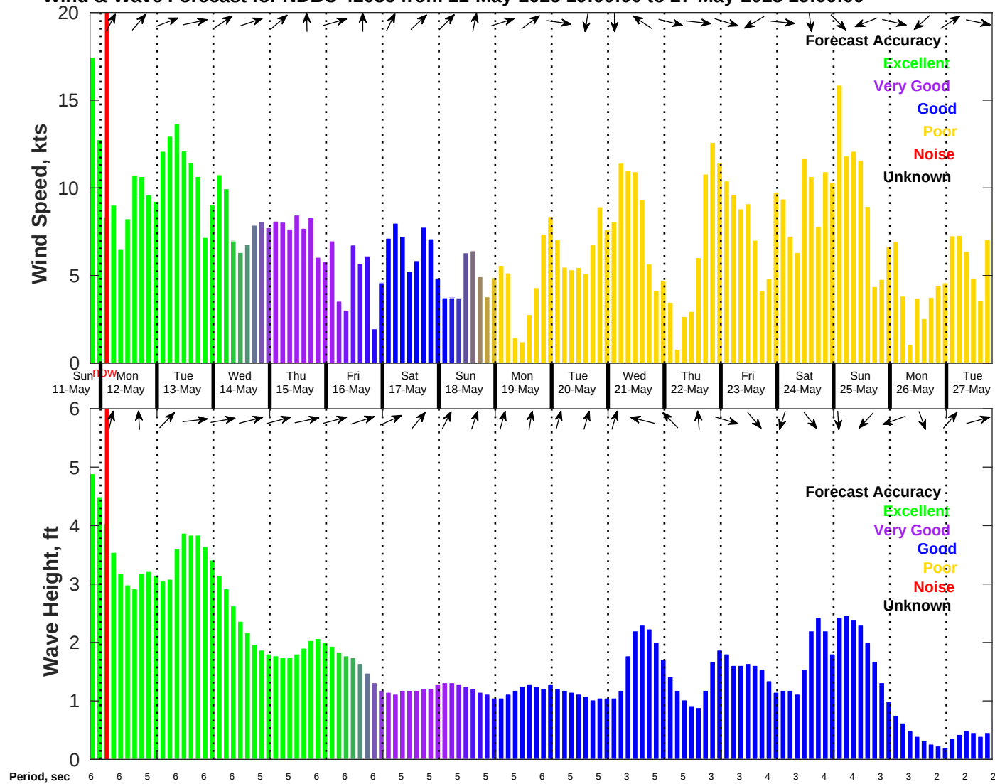
Wind & Wave Forecast for NDBC 42036 from 11-May-2025 19:00:00 to 27-May-2025 19:00:00
