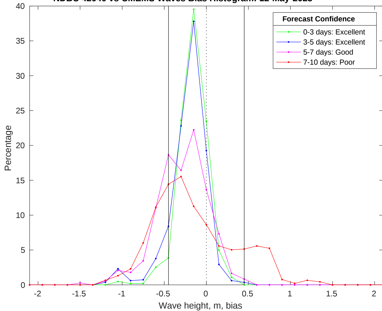
NDBC 42040 vs CMEMS Waves Bias Histogram: 12-May-2025
