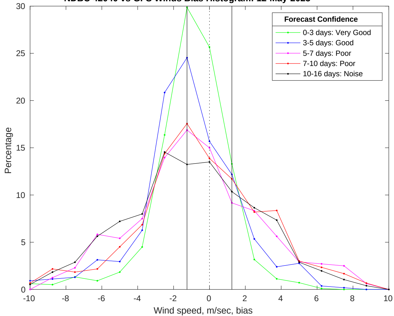
NDBC 42040 vs GFS Winds Bias Histogram: 12-May-2025
