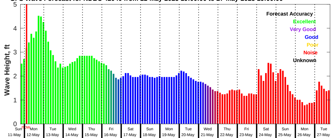
GFS Wave Forecast for NDBC 42040 from 11-May-2025 19:00:00 to 27-May-2025 19:00:00
