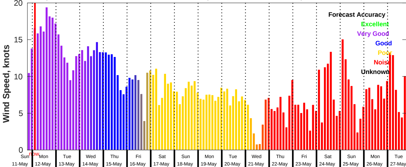
GFS Wind Speed Forecast for NDBC 42040 from 11-May-2025 19:00:00 to 27-May-2025 19:00:00
