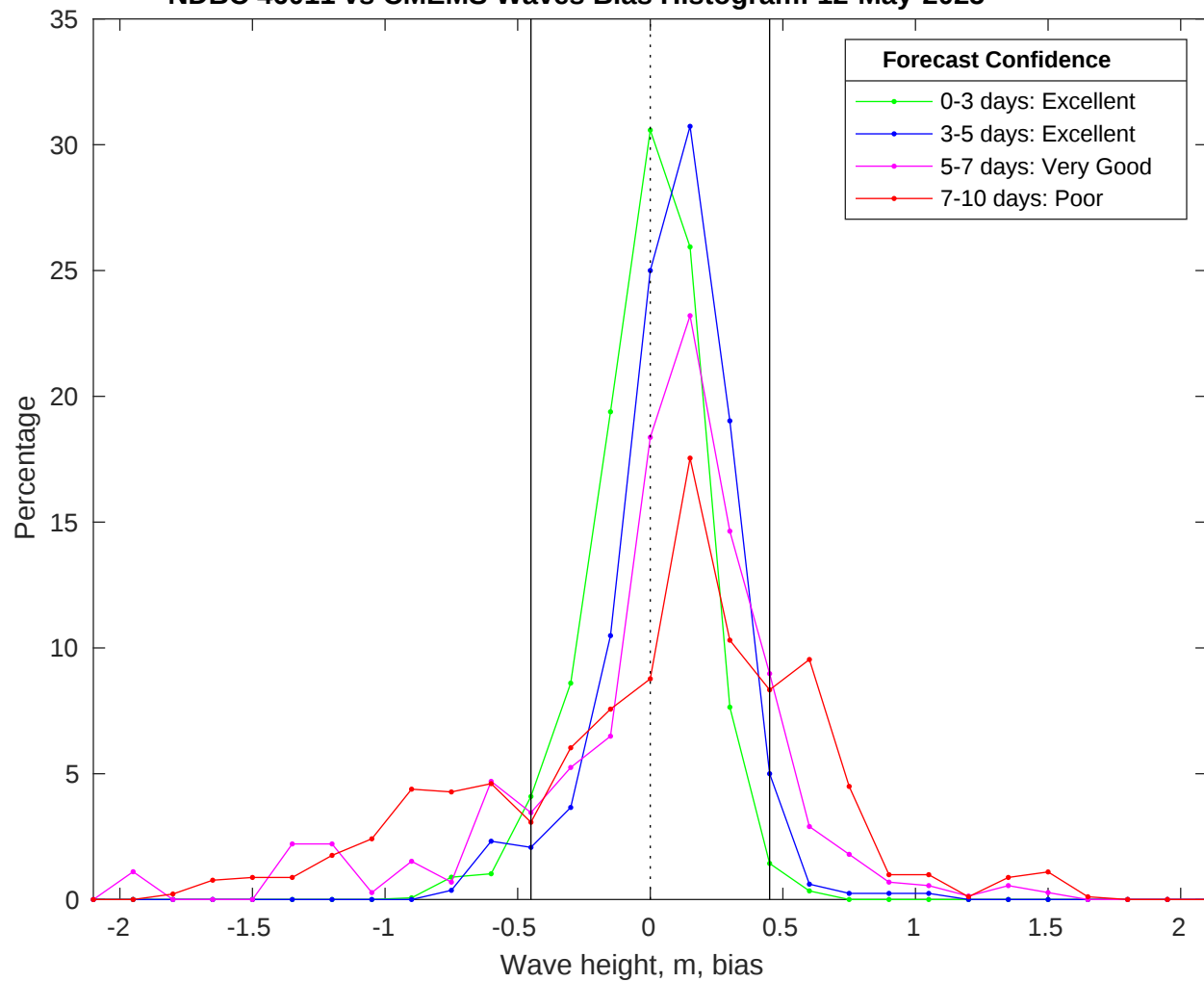
NDBC 46011 vs CMEMS Waves Bias Histogram: 12-May-2025
