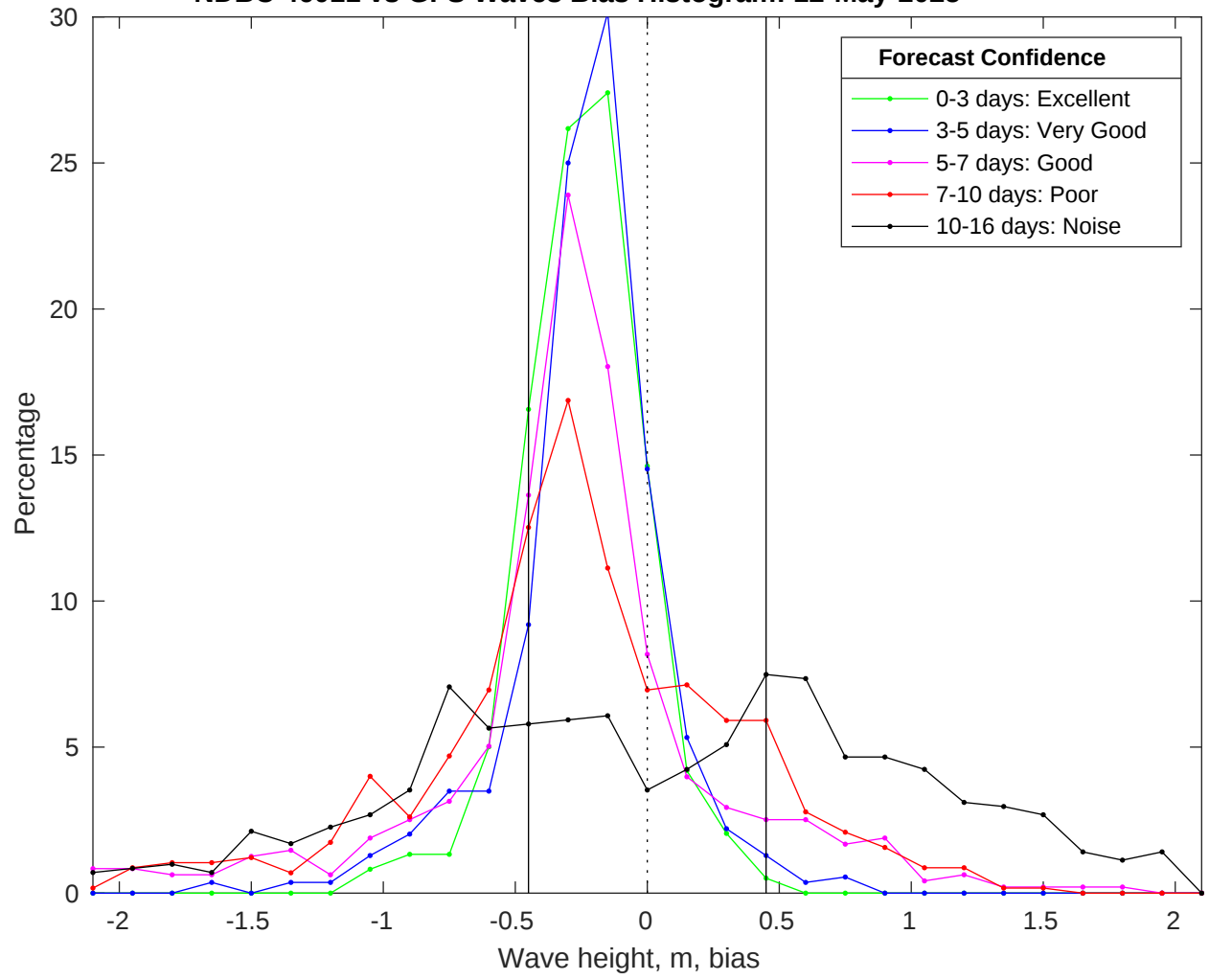
NDBC 46011 vs GFS Waves Bias Histogram: 12-May-2025
