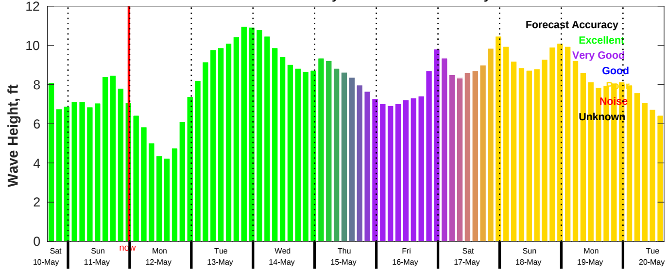
CMEMS Wave Forecast for NDBC 46011 from 10-May-2025 16:00:00 to 20-May-2025 16:00:00
